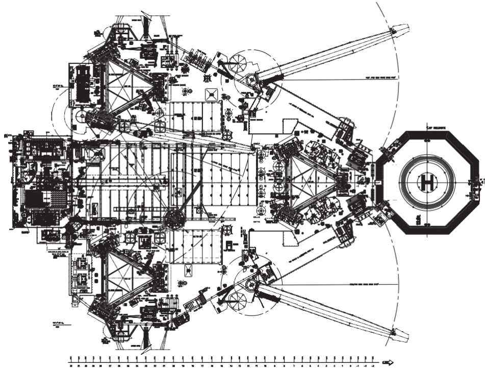
MAIN DECK ARRANGEMENT
